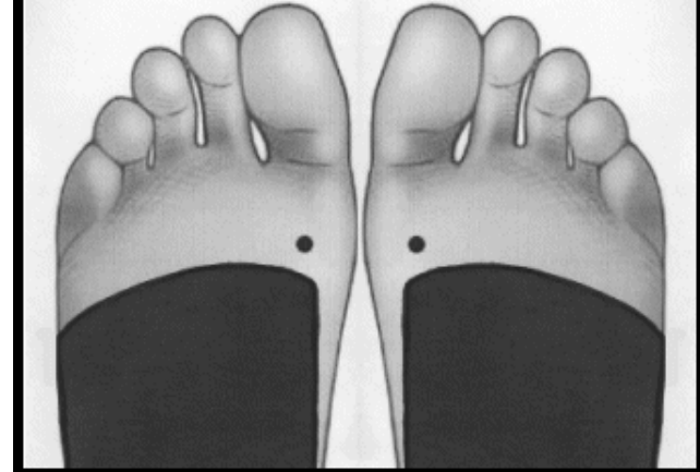
BISECT 1st
