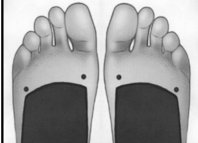
BISECT 1-5
