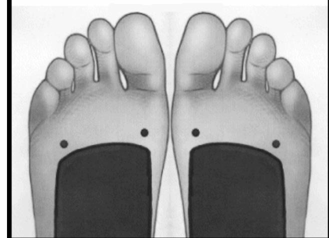
BISECT 1-4
